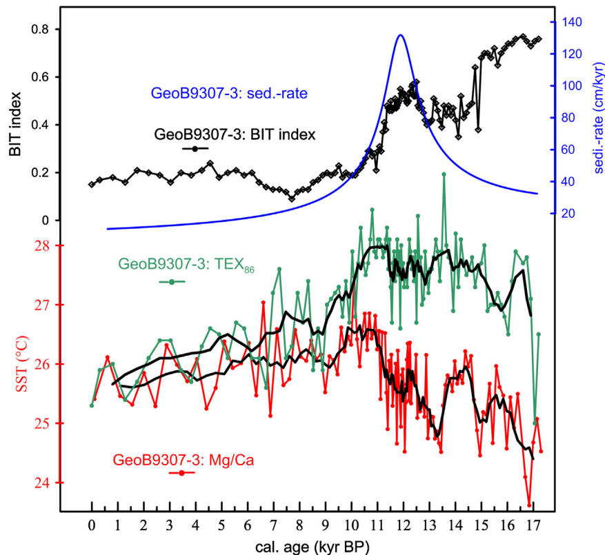
Fig. 5. Comparison of SST estimates based on Mg/Ca (this study, red line) and \text{TEX}_{86} (Schefuß et al. (2011), green line) analyzed in GeoB9307-3. Black lines indicate 5-point running average of SST estimates. Sedimentation rate of GeoB9307-3 core sediment is also shown (blue line). The variability of terrestrial organic matter (TOM), as indicated by the BIT-index, is shown (Schefuß et al., 2011) (black line). At times of significantly elevated input of TOM, the \text{TEX}_{86} -derived SST is higher by up to \sim 3^\circ\text{C} as compared to the Mg/Ca-based SST. Throughout the Holocene, when the input of TOM was very low, the \text{TEX}_{86} -derived and Mg/Ca-based SST estimates are in generally better agreement, although still offset. (For interpretation of the references to color in this figure legend, the reader is referred to the web version of this article.)
