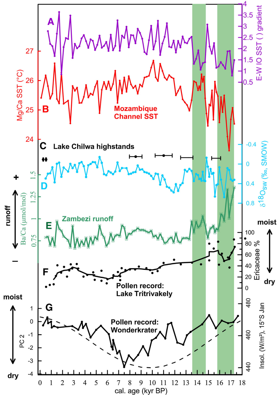
Fig. 8. Comparison of paleo-environmental and thermal changes in southeastern Africa and in the tropical Indian Ocean. A) Changes in zonal Indian Ocean SST gradient established using the difference between the eastern (Xu et al., 2008: 13°4.95'S, 121°47.27'E) and western Indian Ocean SST records (this study). To establish the zonal SST gradient, the Xu et al. (2008) record was digitally resampled at a constant interval of 200 years. B) SST record from the Mozambique Channel. C) Reconstructed intervals of Lake Chilwa highstands (Thomas et al., 2009). D) Temperature and sea level corrected \delta^{18}\text{O} of seawater. E) Relative runoff estimate of Zambezi runoff based on Ba/Ca analysis in tests of the planktonic foraminifera G. ruber . F) Pollen record (5-point running average) from Lake Tritrivakely in Madagascar indicating changes in moisture availability over the riverine and wind catchment of the lake (Williamson et al., 1998). G) Principal component (PC) analysis of pollen assemblage from Wonderkrater in South Africa (Scott et al., 2012). Dotted line: January (15th) insolation at 15°S (Berger and Loutre, 1991). Green shaded areas indicate wet phases in the Zambezi basin, as suggested by the Ba/Ca record and weakened east–west Indian Ocean SST gradient. (For interpretation of the references to color in this figure legend, the reader is referred to the web version of this article.)
