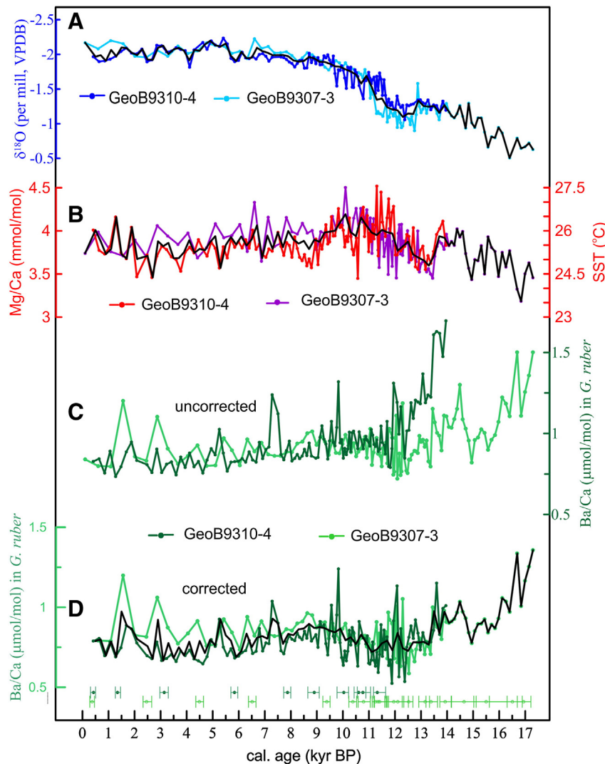
Fig. 4. Proxy parameters analyzed in G. ruber white (250–300 μm). A) \delta^{18}\text{O} , B) Mg/Ca and Mg/Ca-SST estimates. C) Uncorrected and D) corrected Ba/Ca (see text). Black lines in A, B), and D) between 0 and 14 kyr BP indicate binned data of GeoB9310-4 and GeoB9307-3 (bin size 200 yr); for sections older than 14 ka cal BP, black lines indicate in A, B), and D) unbinned data of GeoB9307-3. Green dots along the x-axis indicate ^{14}\text{C} -date-based age model control points and their uncertainties (Table 1). (For interpretation of the references to color in this figure legend, the reader is referred to the web version of this article.)
