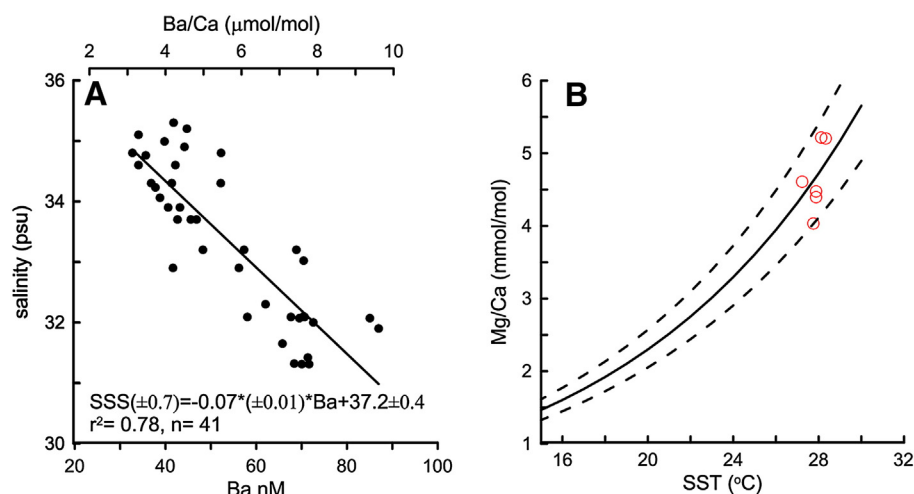
Fig. 2. A) Relationship between seawater Ba (Ba/Ca) and sea surface salinity in Mozambique Channel surface water (samples taken in February/March, 2008). Note that samples with low salinity and high Ba are from runoff-influenced sites (see Fig. 1). B) Mg/Ca in G. ruber tests (300–400 μm) from plankton tows plotted versus temperature (0–30 m) measured via CTD between February 29th and March 9th, 2008. Continuous and dashed lines indicate the global calibration curve and its uncertainty, respectively (Dekens et al., 2002; Anand et al., 2003).
