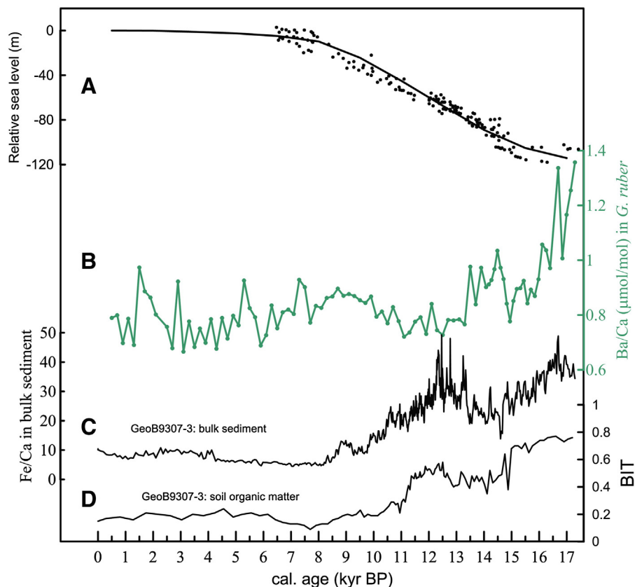
Fig. 7. A) Black line indicates eustatic sea level changes derived from benthic foraminiferal \delta^{18}\text{O} (Waelbroeck et al., 2002) and black dots relative sea level changes based on corals from several sites compiled by Clark et al. (2009) and from Tahiti (Deschamps et al., 2012). B) Ba/Ca analyzed in tests of the planktonic foraminifera G. ruber (250–300 \mu\text{m} ) from cores GeoB9307-3 and GeoB931904 (composited and binned: bin size 200 yr). C) Fe/Ca ratios analyzed in bulk sediment using XRF-scanning (Schefuß et al., 2011). D) Branched and isoprenoid tetraether (BIT) index used as indicator of relative soil organic matter contributions (Schefuß et al., 2011).
