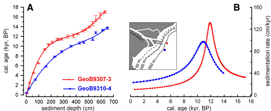
Fig. 3. A) Radiocarbon-based age model control points of GeoB9307-3 (red diamonds) and GeoB9310-4 (blue dots) plotted versus sampling sediment depth. The final age model is based on fourth order polynomial fits: age (cal. kyr) = -3E-10x(\text{depth})^4 + 5E-7x(\text{depth})^3 - 0.0003x(\text{depth})^2 + 0.1043x(\text{depth}) - 0.2102 for GeoB9307-3 and age (cal. kyr) = 7E-7x(\text{depth})^4 - 3E-8x(\text{depth})^3 - 5E-5x(\text{depth})^2 + 0.0437x(\text{depth}) + 0.2892 for GeoB9310-4, where depth is sediment depth in cm. B) Changes in sedimentation rate in GeoB9307-3 and GeoB9310-4 plotted versus calendar age model. Inset shows location of GeoB9307-3 (red diamond) and GeoB9310-4 (blue dot) relative to the Zambezi river mouth and paleo-Chinde-Zambezi Channel (Beiersdorf et al., 1980; Schulz et al., 2011). (For interpretation of the references to color in this figure legend, the reader is referred to the web version of this article.)
