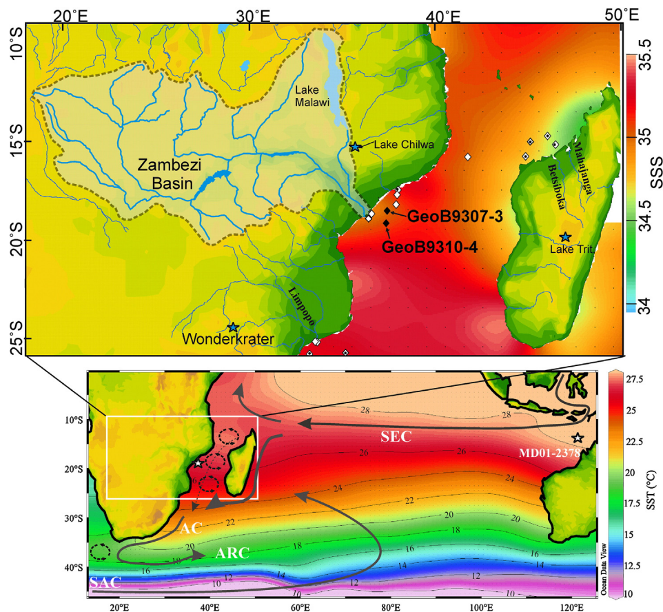
Fig. 1. Sampling locations and annually averaged hydrographic characteristics in the southern tropical Indian Ocean. Upper panel shows the Zambezi basin, core locations (black diamonds) of GeoB9307-3 ( 18^\circ33.90'\text{S} , 37^\circ22.80'\text{E} , water depth 542 m) and GeoB9310-4 ( 19^\circ12.11'\text{S} , 37^\circ02.49'\text{E} , water depth 543 m), sites of seawater sampling (white diamonds), sites of foraminifer sampling from the water column (black dots in white diamonds), and annual sea surface salinity pattern in the Mozambique Channel and off the Zambezi River (Locarnini et al., 2010). Lower panel shows annually averaged SST (Locarnini et al., 2010) and surface currents (Schott et al., 2002) that are of relevance for heat and salinity exchange in the tropical and southern Indian Ocean. SEC: Southern Equatorial Current, AC: Agulhas Current, ARC: Agulhas Return Current, SAC: South Atlantic Current. Location of MD01-2378 (Xu et al., 2008) in the eastern Indian Ocean is also indicated.
