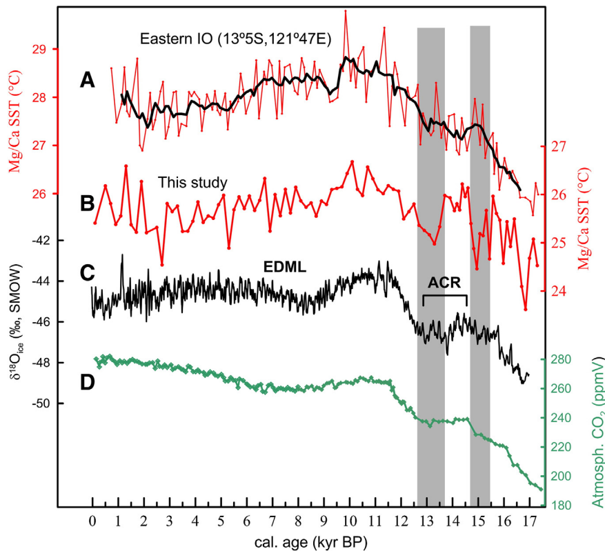
Fig. 6. SST estimates based on Mg/Ca analysis in tests of the planktonic foraminifera G. ruber from (A) the eastern tropical Indian Ocean (Xu et al., 2008) and (B) Mozambique Channel (this study, binned) and plotted versus calendar age (kyr BP); the black line in A indicates a 5-point running average. Gray shaded areas indicate phases of low SST in the Mozambique Channel. C) Shows \delta^{18}\text{O} time series analyzed in Dronning Maud Land (Antarctica) (EDML) ice core (EPICA-Community-members, 2006). D) Atmospheric \text{CO}_2 analyzed in Dome Concordia ice core (Antarctica) (Monnin et al., 2001), 8–17.5 kyr synchronized to GICC05 age scale (Lourantou et al., 2010).
